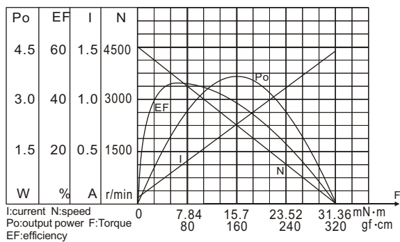
RS-395126000 CHARACTERISTICS
