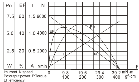
RS-395246000 CHARACTERISTICS
