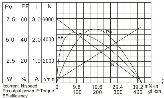
RS-395126000 CHARACTERISTICS
