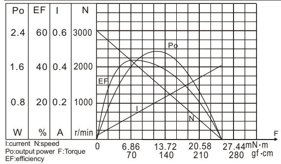
RS-395244500 CHARACTERISTICS
