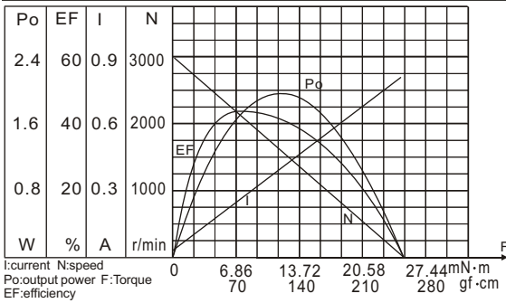
RS-395124500 CHARACTERISTICS
