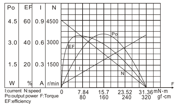
RS-395246000 CHARACTERISTICS
